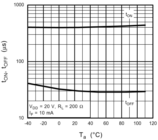
Fig. 14.10 t_{ON} , t_{OFF} - T_a
