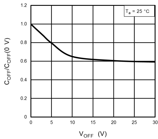
Fig. 14.13 C_{OFF}/C_{OFF} - T_a
