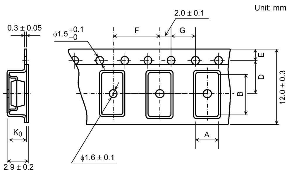
Symbol Dimension Remark A 4.0 — B 7.6 — D 5.5 Center line of embossed cavity and sprocket hole E 1.75 Distance between tape edge and sprocket hole center F 8.0 Cumulative error +0.1/-0.3 (max) per 10 empty cavities holes G 4.0 Cumulative error +0.1/-0.3 (max) per 10 sprocket holes K 0 2.6 Internal space
