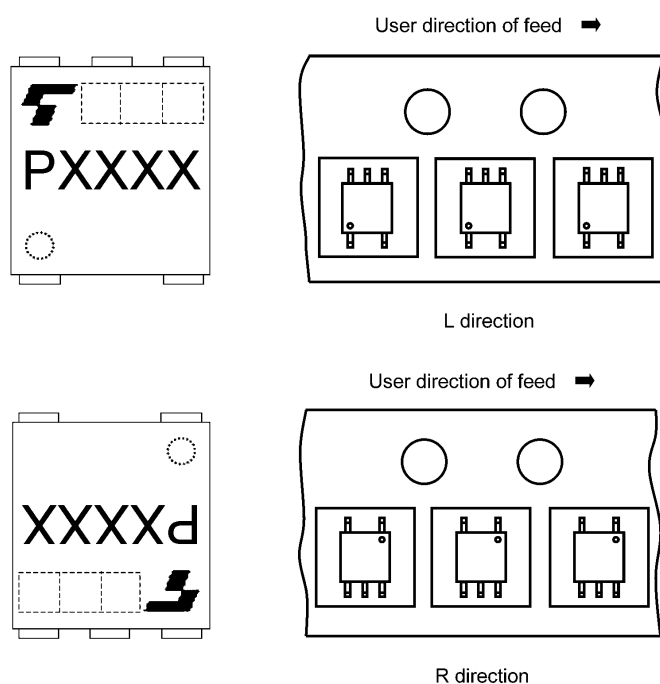
Device Orientation
