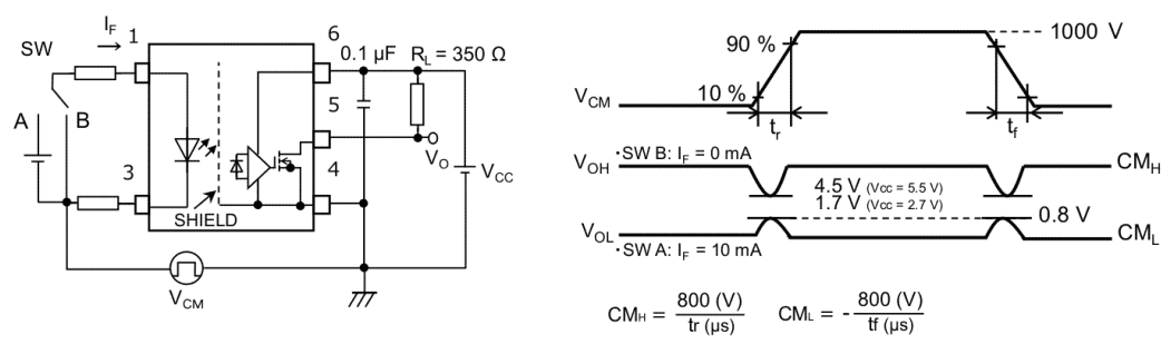
Fig. 12.1.7 Common-Mode Transient Immunity Test Circuit and Waveform
