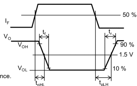
Fig. 12.1.6 Switching Time Test Circuit and Waveform
