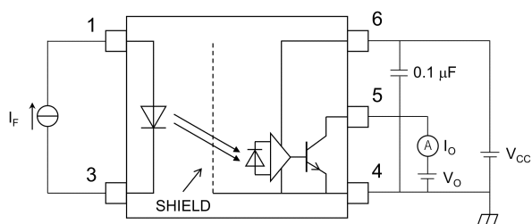
Fig. 12.1.5 I_O Test Circuit
