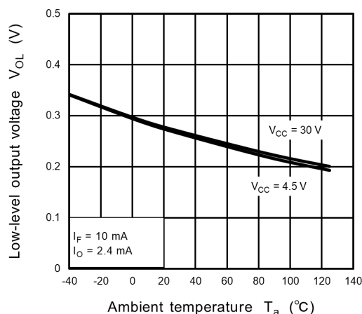
Fig. 12.2.8 V_{OL} - T_a
