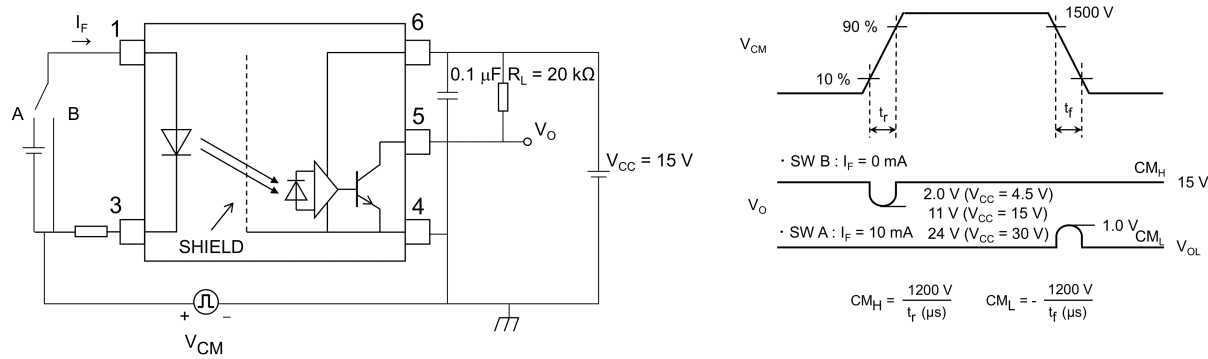
Fig. 12.1.7 Common-Mode Transient Immunity Test Circuit and Waveform
