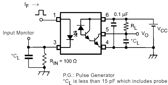
Fig. 12.1.1 Switching Time Test Circuit and Waveform
