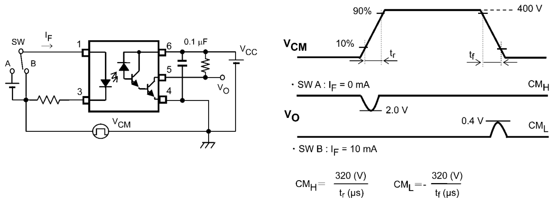
Fig. 12.1.2 Common-Mode Transient Immunity Test Circuit and Waveform
