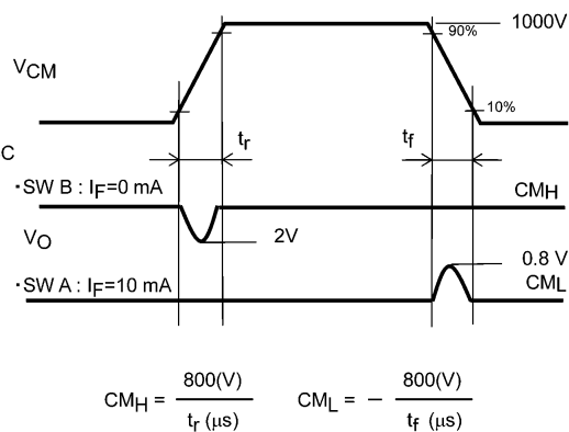
Fig. 12.1.6 Common-Mode Transient Immunity and Waveform
