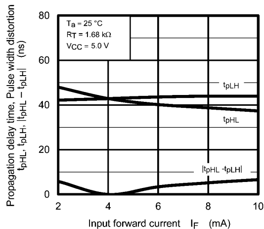
Fig. 12.2.13 t_{pHL} , t_{pLH} , |t_{pHL} - t_{pLH}| - I_F
