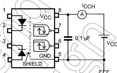
Fig. 12.1.4 ICCCH Test Circuit
