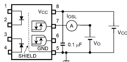
Fig. 12.1.5 IOSL Test Circuit
