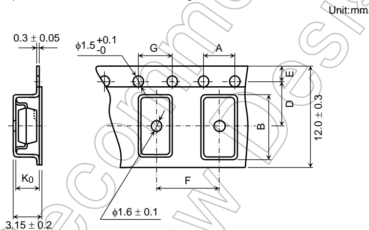
Figure 2 Tape Forms
