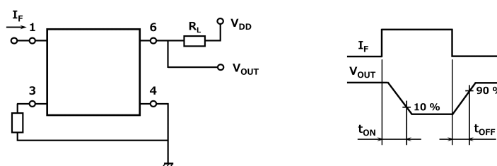
Fig. 13.1 Switching Time Test Circuit and Waveform
