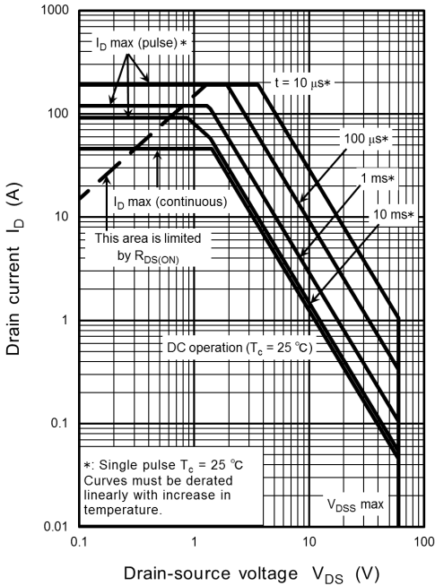
Fig. 8.15 Safe Operating Area (Guaranteed Maximum)
