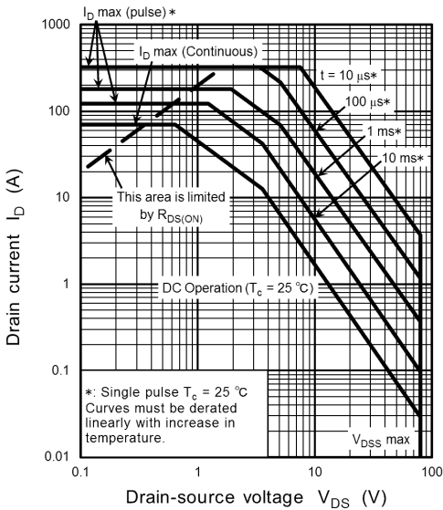
Fig. 8.15 Safe Operating Area (Guaranteed Maximum)
