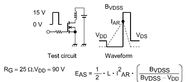
Fig. 8.16 Test Circuit/Waveform
