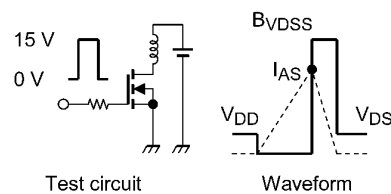
Fig. 9.15 Test Circuit/Waveform
