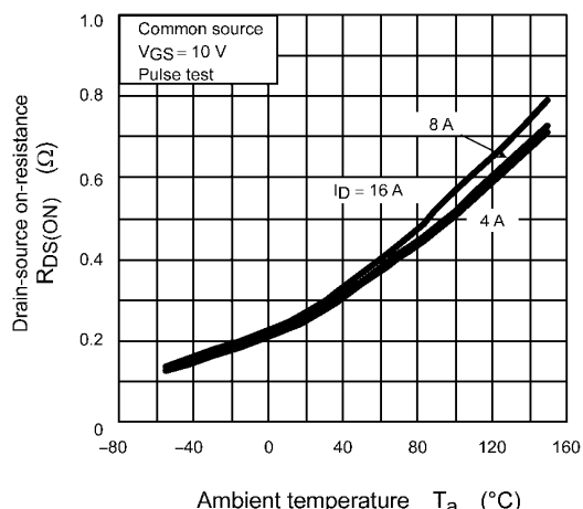
Fig. 8.7 R_{DS(ON)} - T_a
