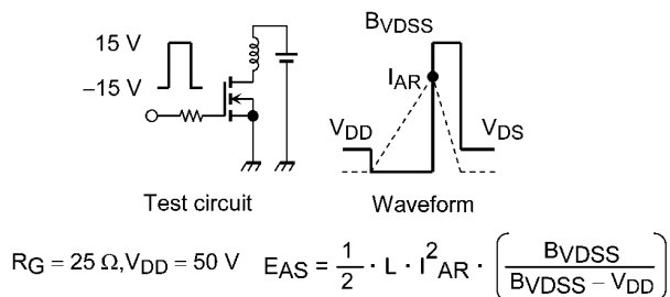
Fig. 8.16 Test Circuit/Waveform
