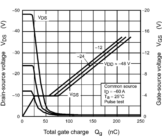
Fig. 8.10 Dynamic Input/Output Characteristics
