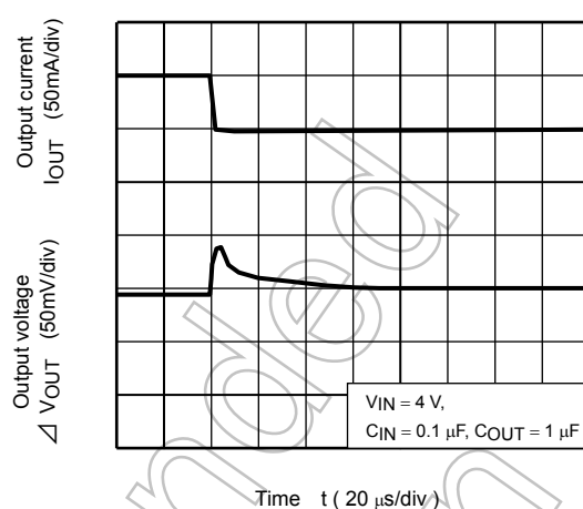
TCR5SB30 ( I_{OUT} = 100\text{m to }50\text{mA} )
