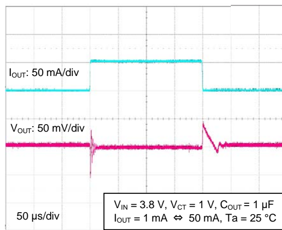
V OUT = 2.8V
