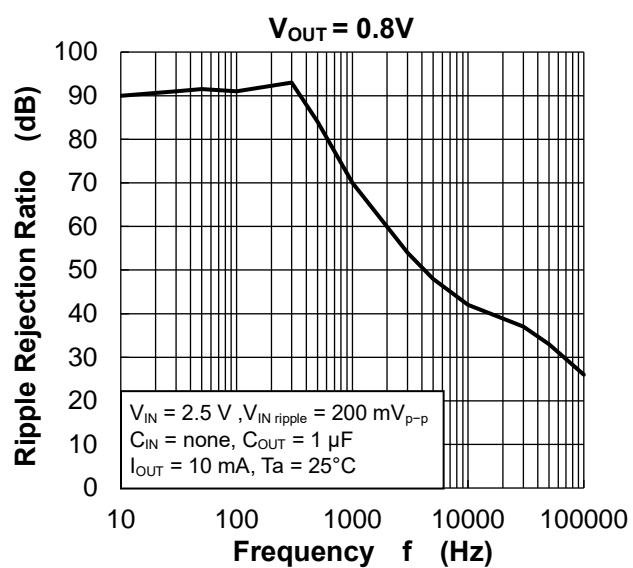
Ripple Rejection Ratio vs. Frequency
