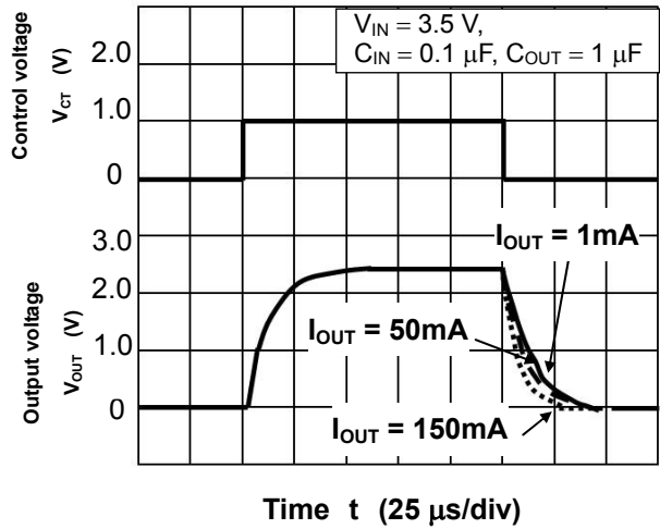
V_{OUT}=2.5V
