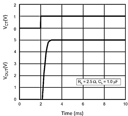
t_{ON} Response
