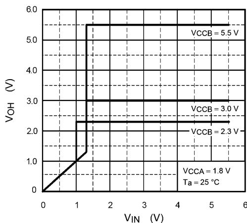
Fig. 14.2 Input/Output Characteristics (Typ.) VCCA = 1.8 V, Ta = 25 °C
