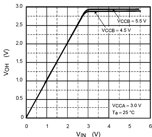
Fig. 15.4 Input/Output Characteristics (Typ.) VCCA = 3.0 V, Ta = 25 °C
