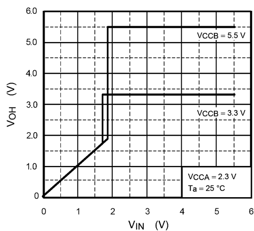
Fig. 14.3 Input/Output Characteristics (Typ.) VCCA = 2.3 V, Ta = 25 °C
