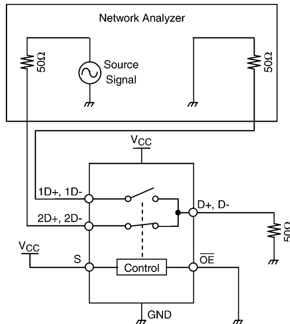
Fig. 11.7 Crosstalk
