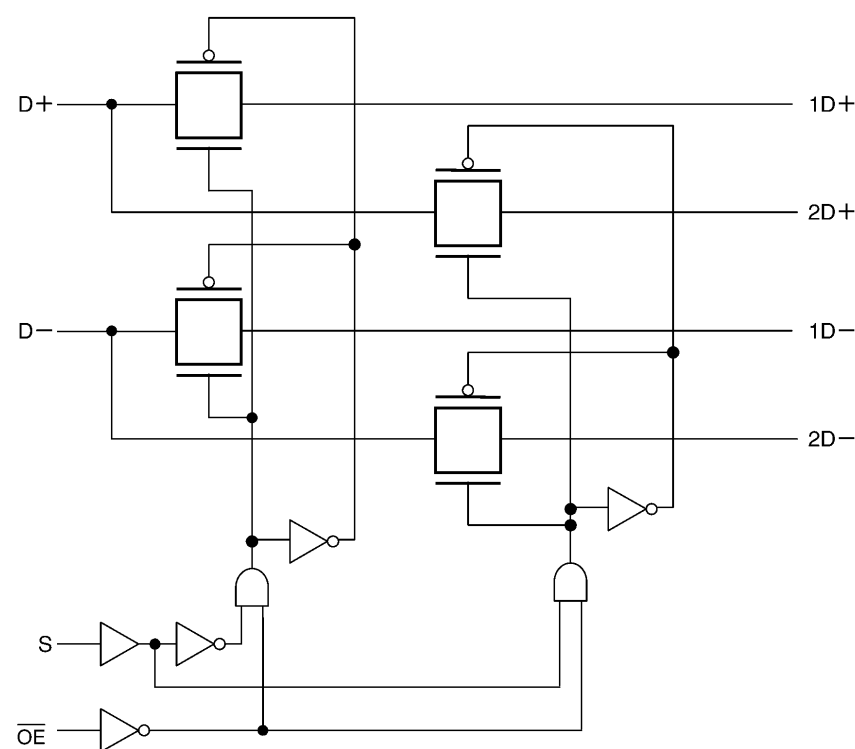
Fig. 6.1 Block Diagram
