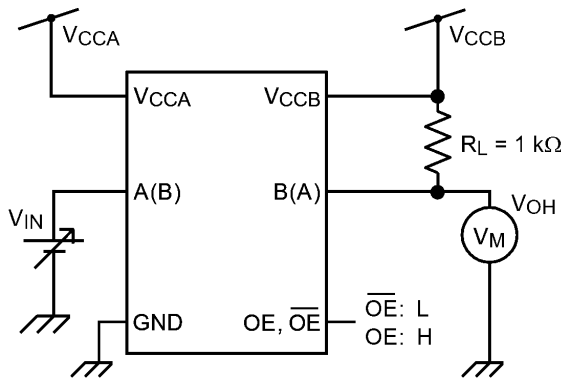
Fig. 15.1 Test Circuit
