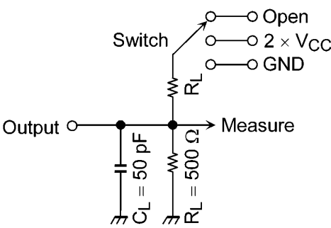
Fig. 11.2.1 AC Test Circuit
