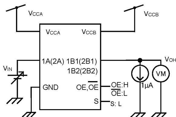
Fig. 16.1 Test Circuit
