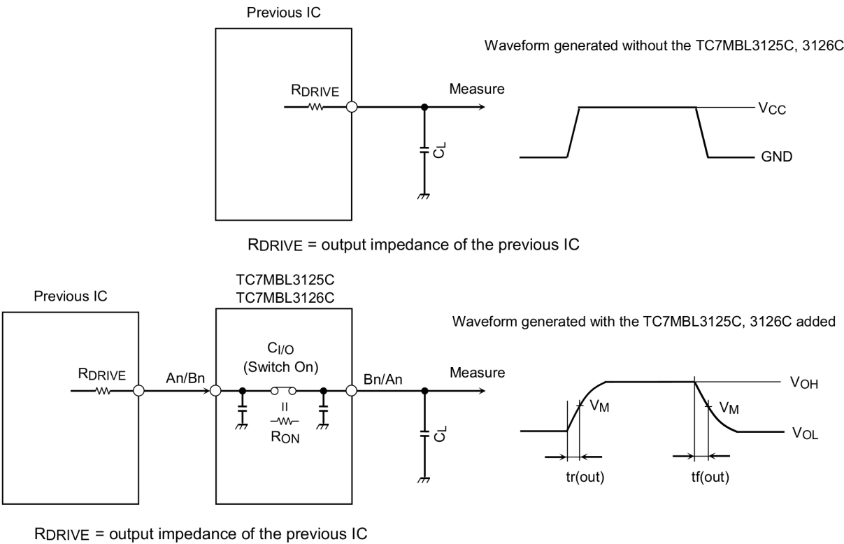
Fig. 12.1 Calculation Circuit
