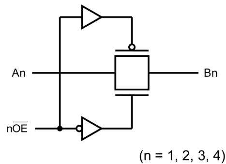
TC7MBL3125CFT
