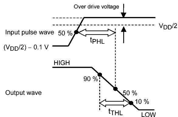
Fig. 10.6 Propagation delay time (H/L) t_{PHL} wave
