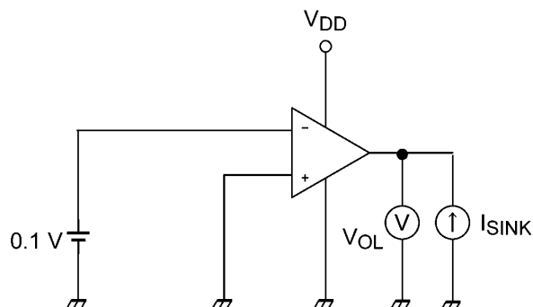
Fig. 10.2 I_{SINK}, V_{OL}
