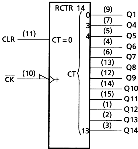
TC74HC4020A
