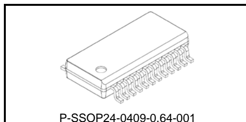
P-SSOP24-0409-0.64-001
