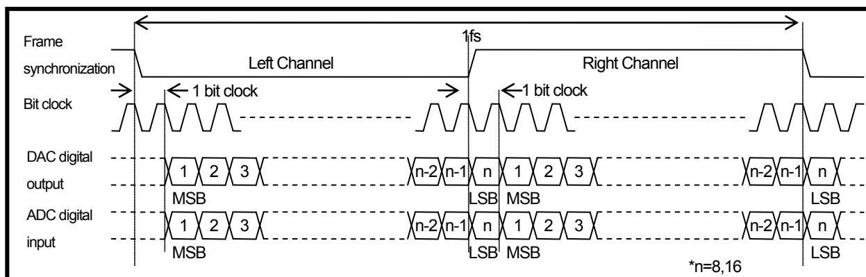
Figure 4-13 I 2 S format
