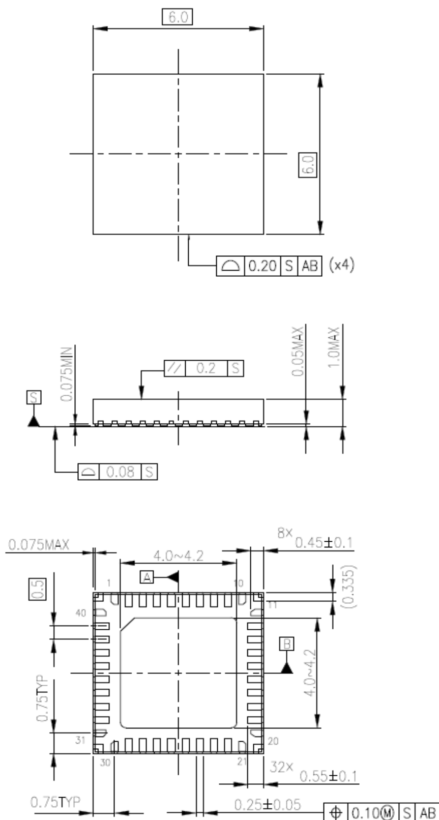
Figure 13.2. Package dimensions TB9054FTG
