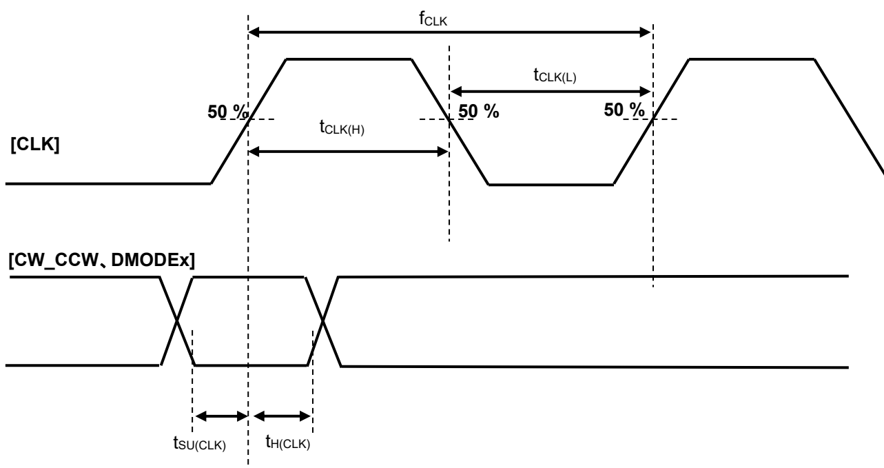
Figure20.2 TB67S589FTG(Relationship between CLK and other control signals)
