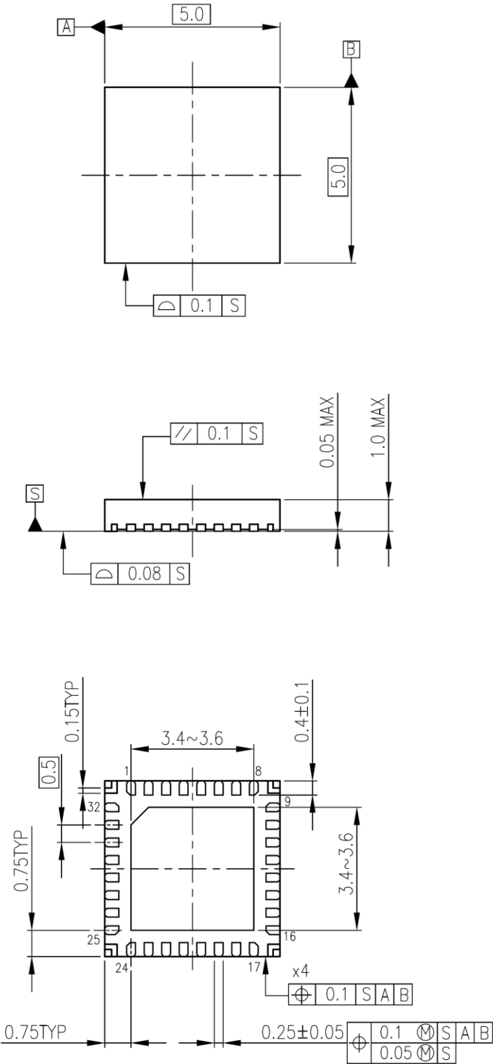
Figure22 Package Dimensions
