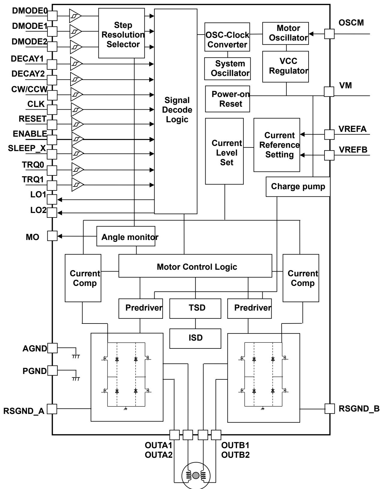
Figure 4 Block diagram
