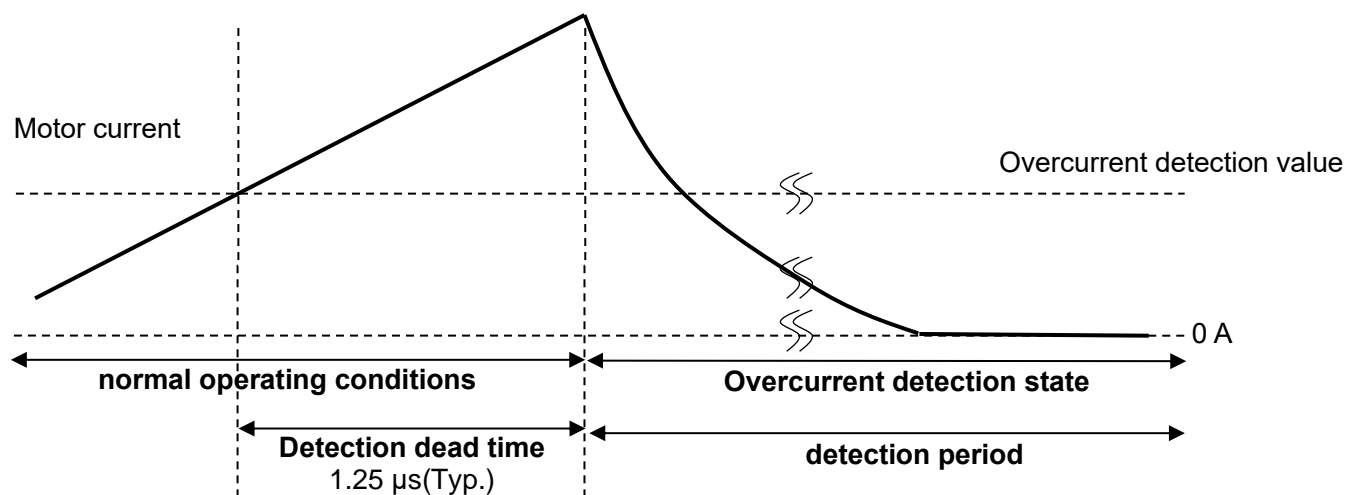
Figure14 Overcurrent detection
