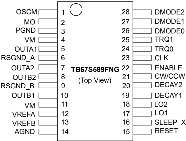
Figure 3 Pin Assignment
