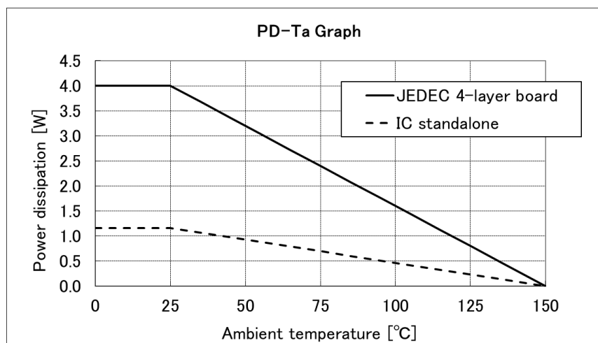
Figure16 PD-Ta graph
