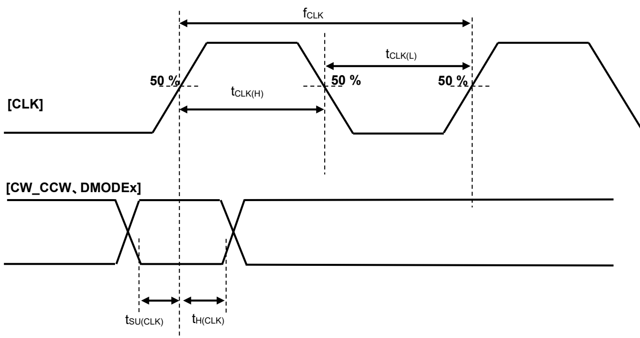
Figure20.2 TB67S589FNG(Relationship between CLK and other control signals)
