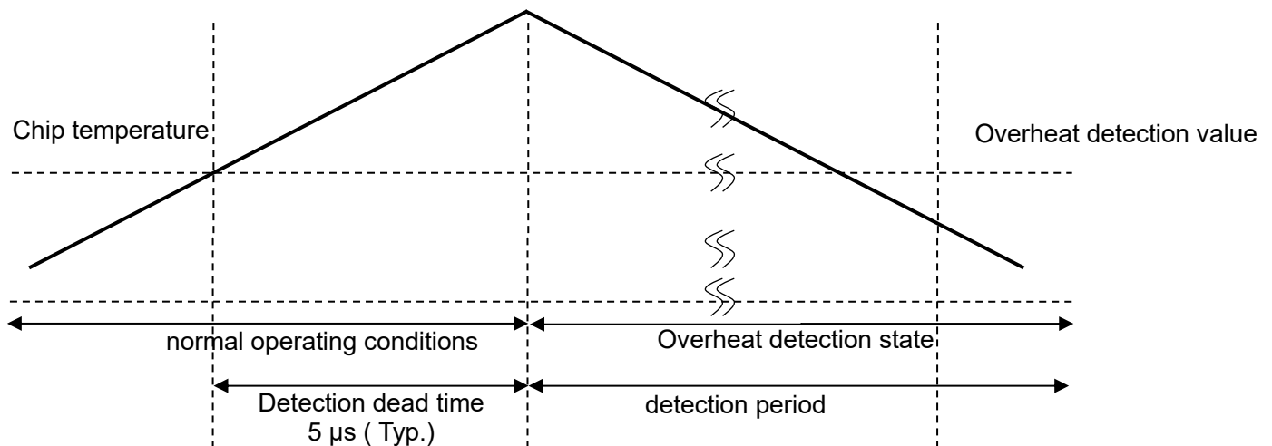
Figure13 Overheat Detection
