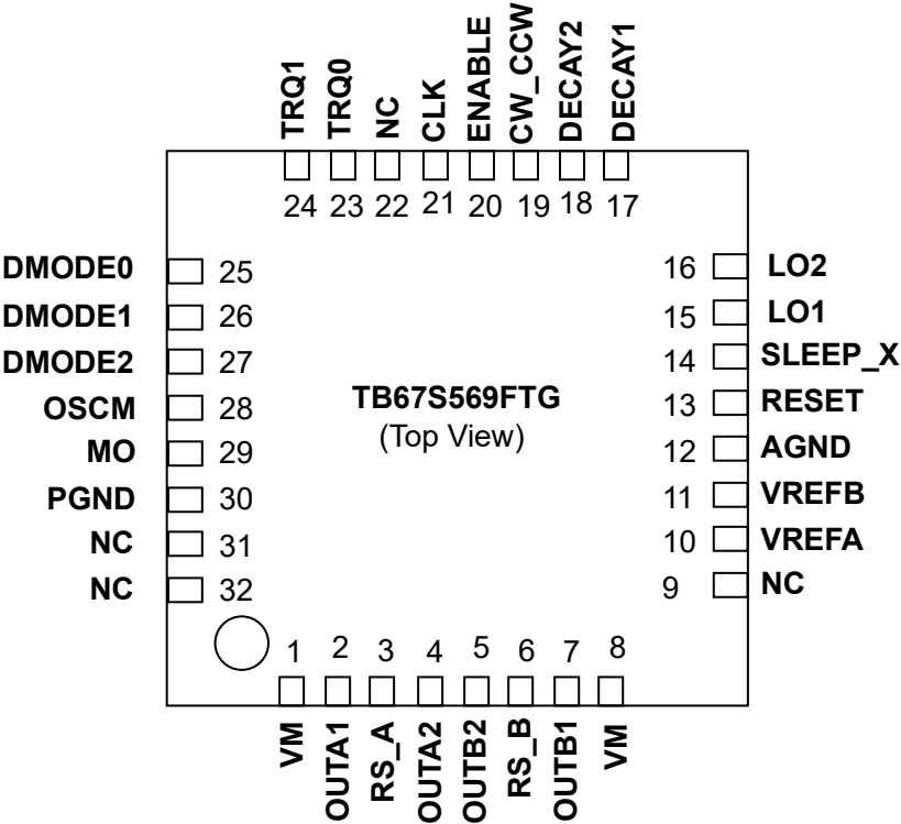
Figure 3 Pin Assignment
