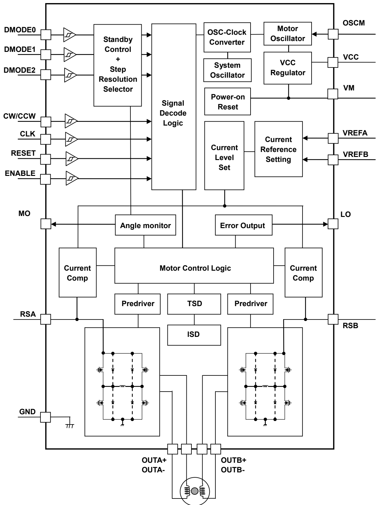
TB67S269 Block diagram
