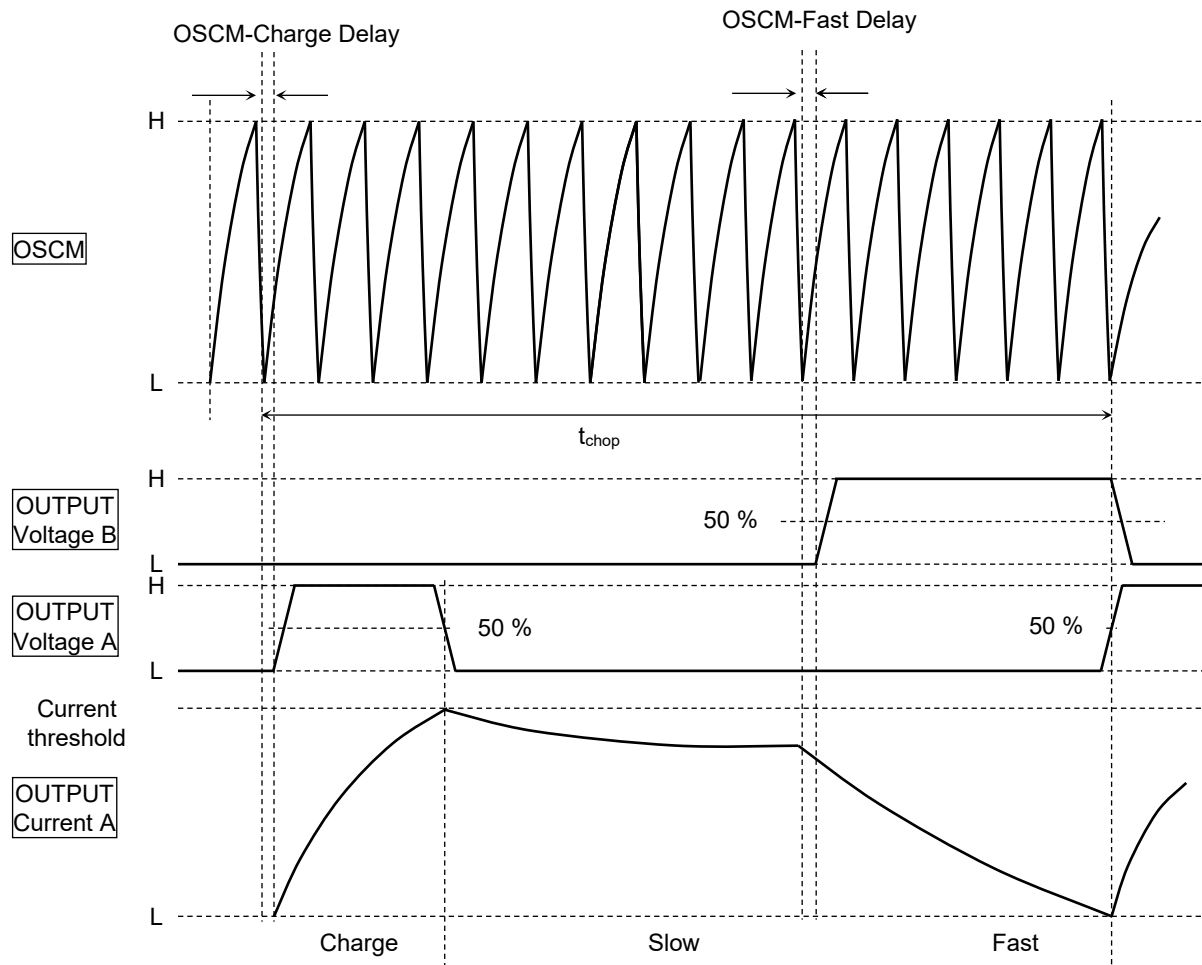
Figure20.1 OSCM-Charge DELAY
