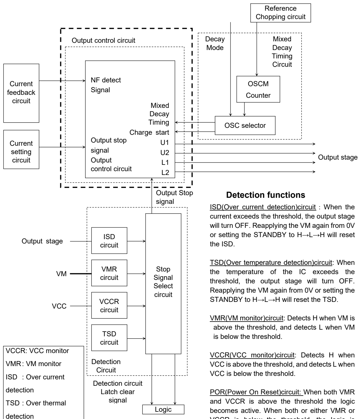
Figure6 Output control circuit current value feedback circuit, current value setting circuit
