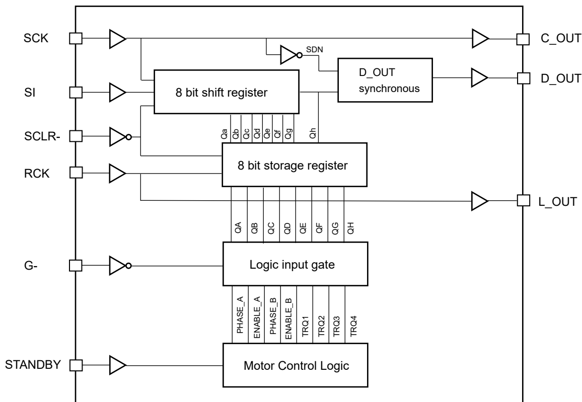
Figure8 Serial control interface (8 bit shift register+8bit storage register)
