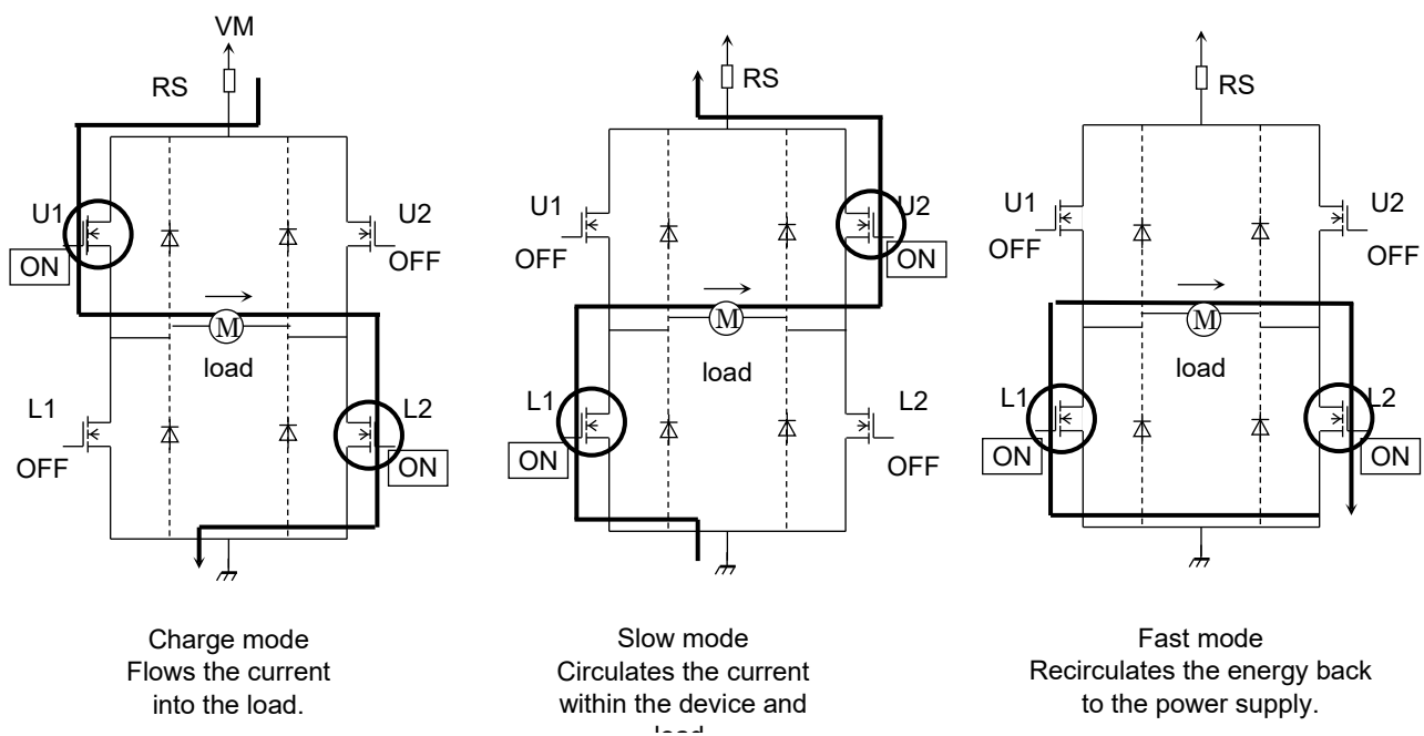
Figure16 Motor output MOSFET operation mode
