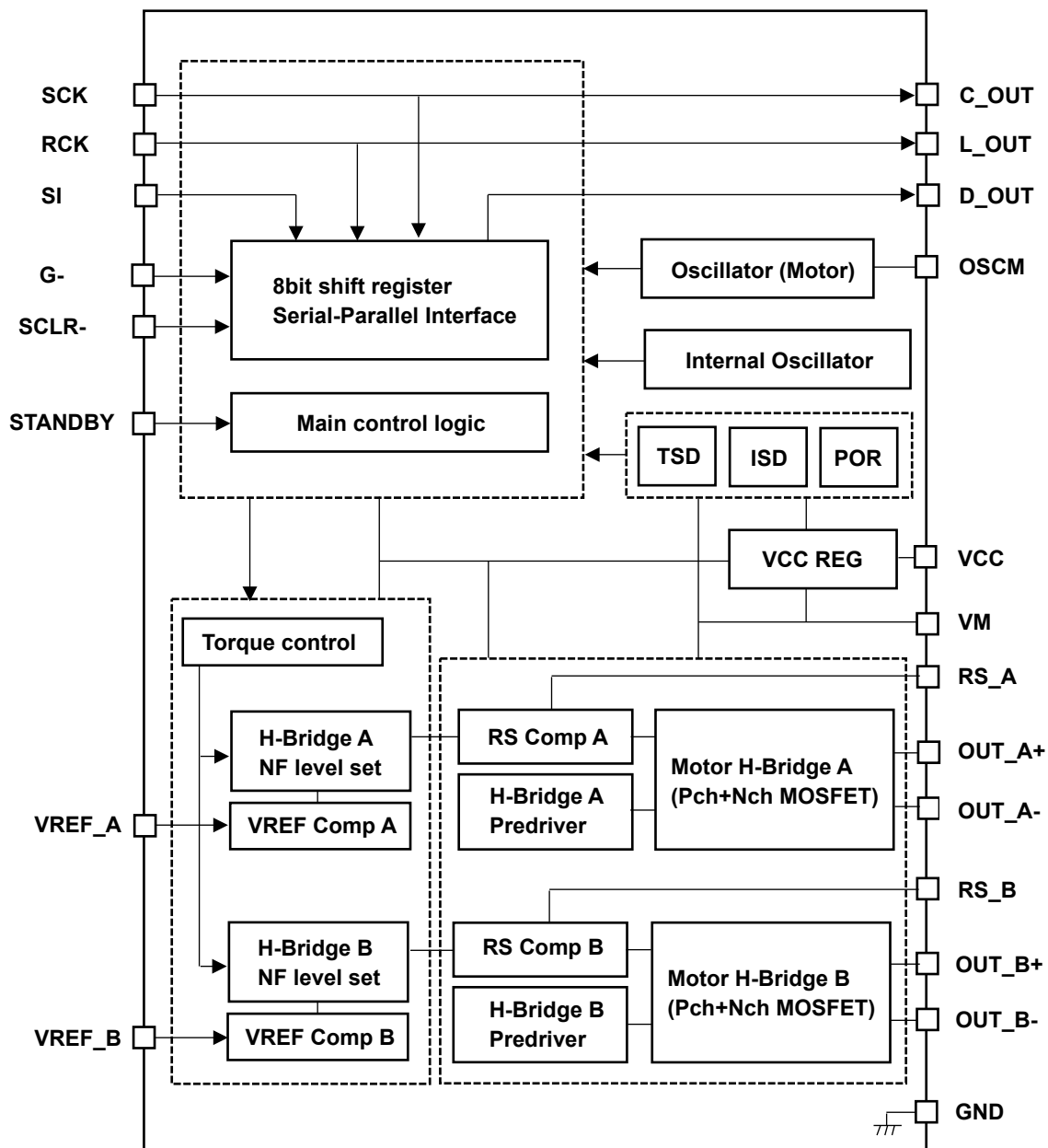
Figure5 Block diagram
