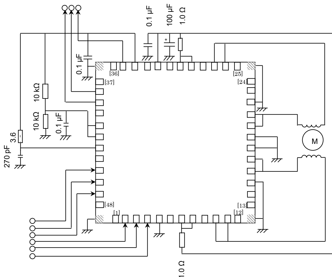
Figure26 TB67S105FTG application circuit
