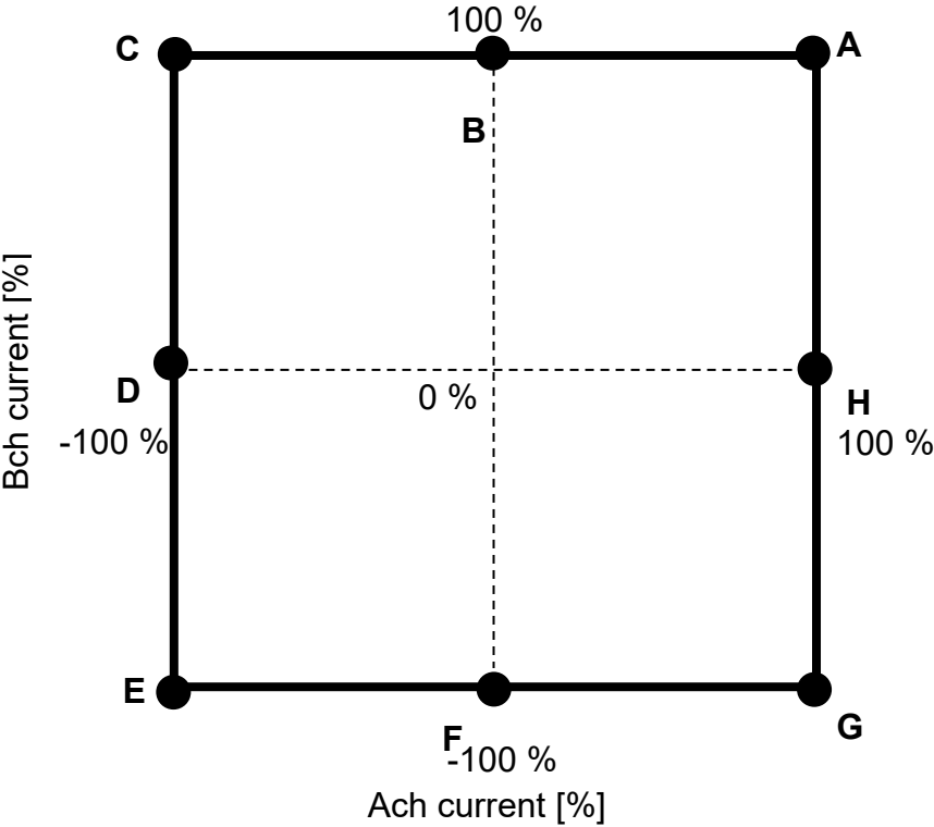
Figure21.2.1 Half step resolution sequence
