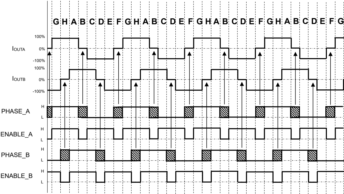
Figure21.2.2 Half step resolution sequence timing chart
