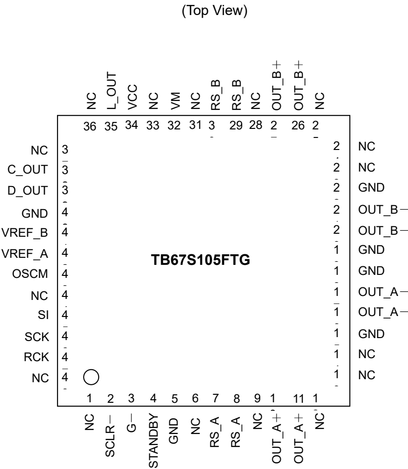
Figure3 Pin assignment
