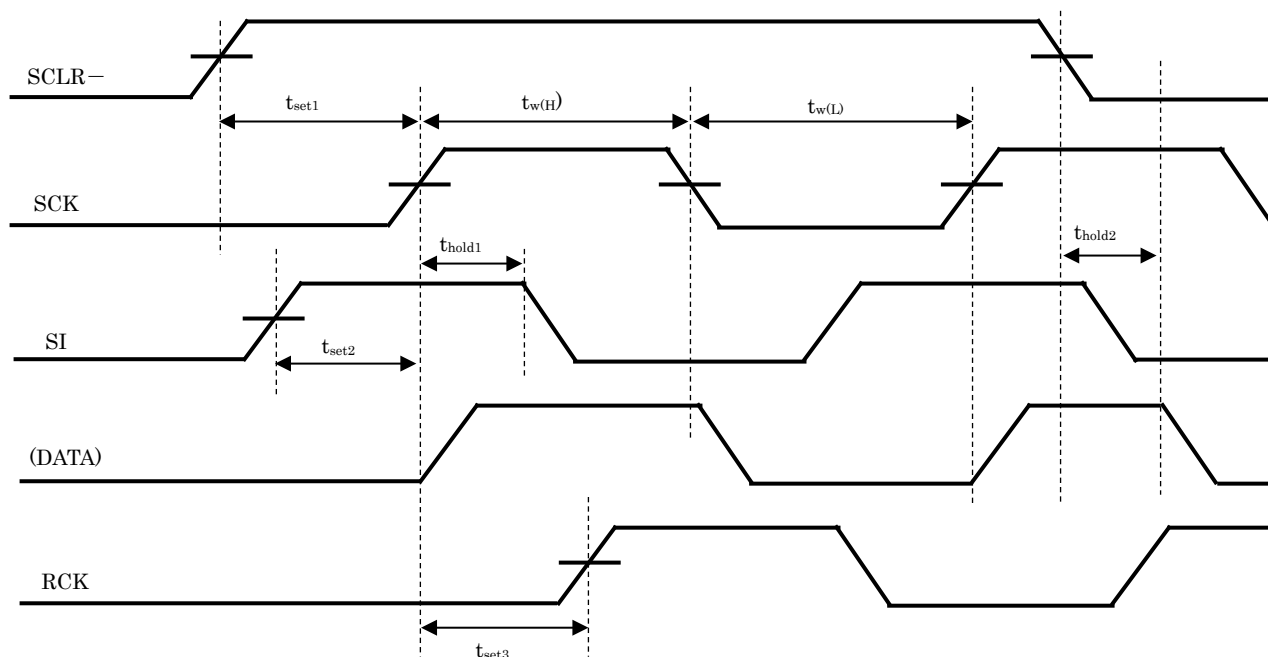
Figure13 AC Electrical Specification Timingchart
