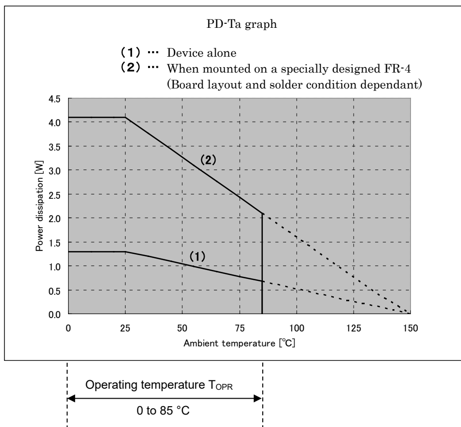
Figure25 (For reference) PD-Ta graph
