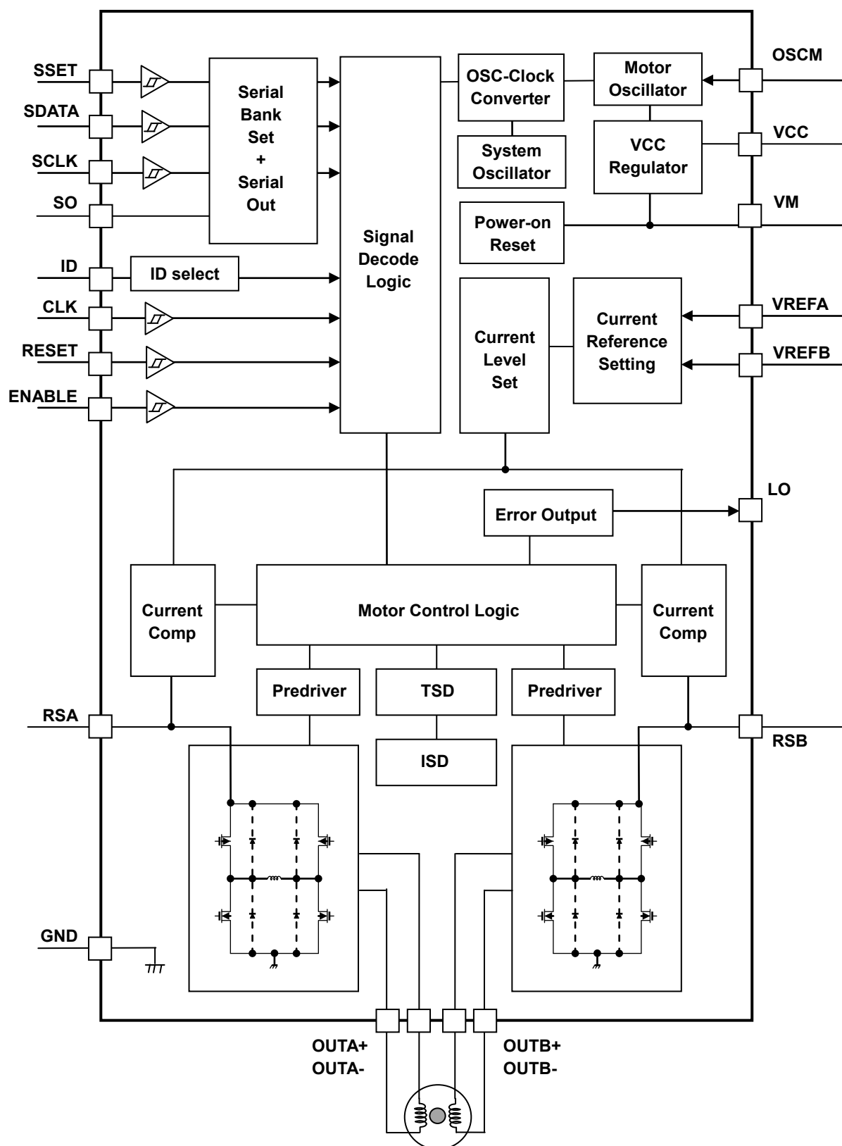
TB67S103A Block diagram
