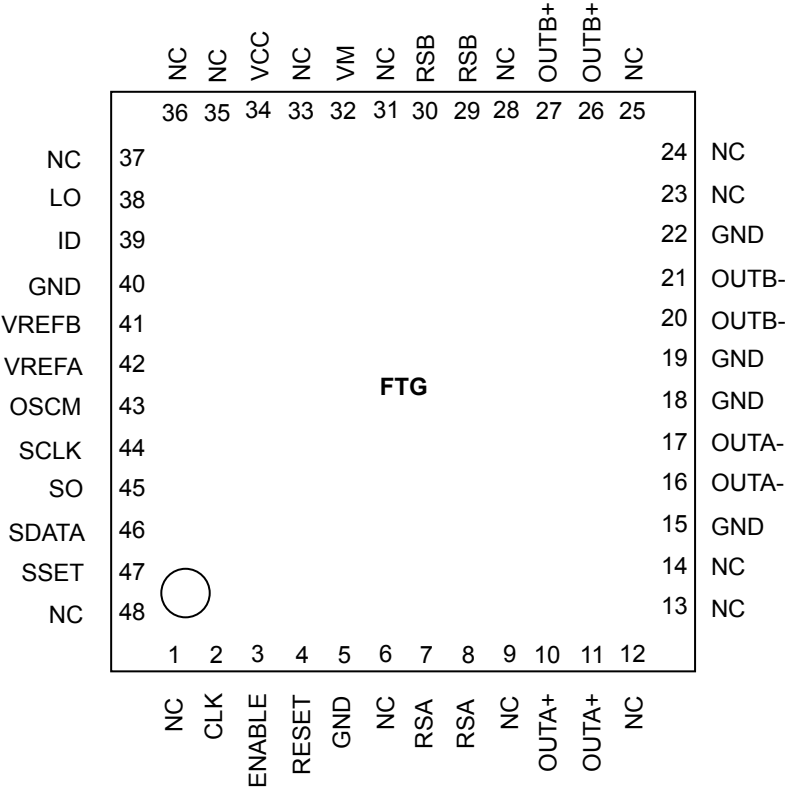
Pin assignment (TB67S103A) (Top View)
