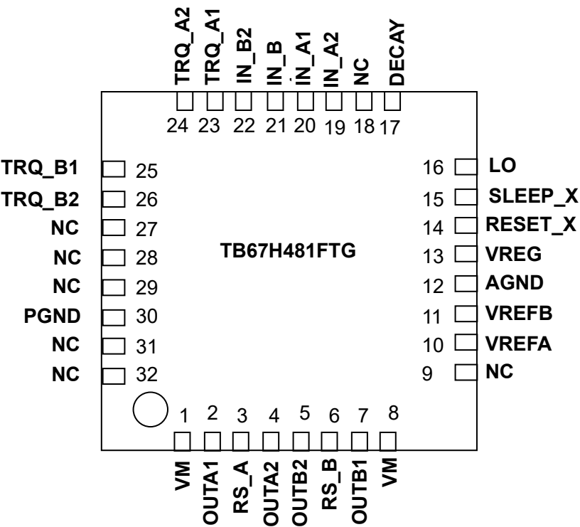
Figure3 Pin Assignment
