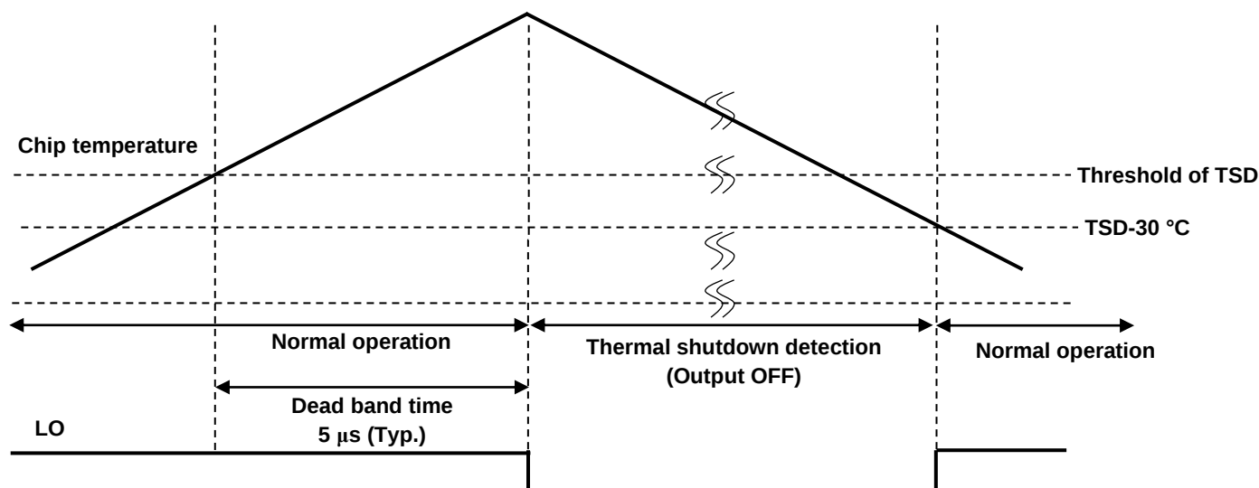
Figure10.1 Thermal shutdown detection timing chart 1
