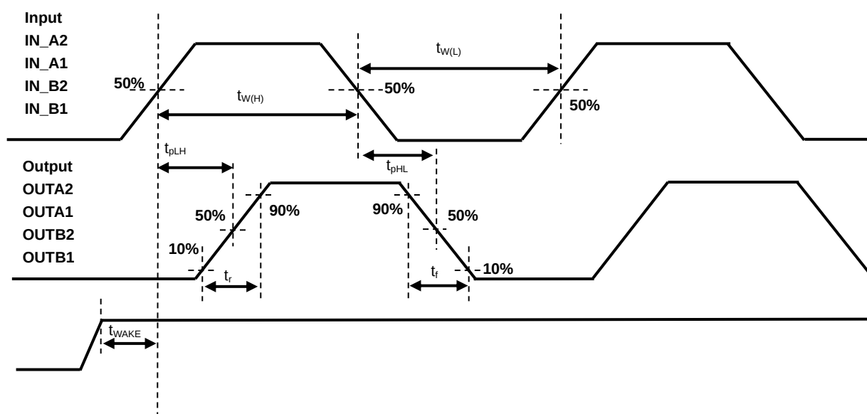
Figure15.1 AC Electrical Specification Timing charts
