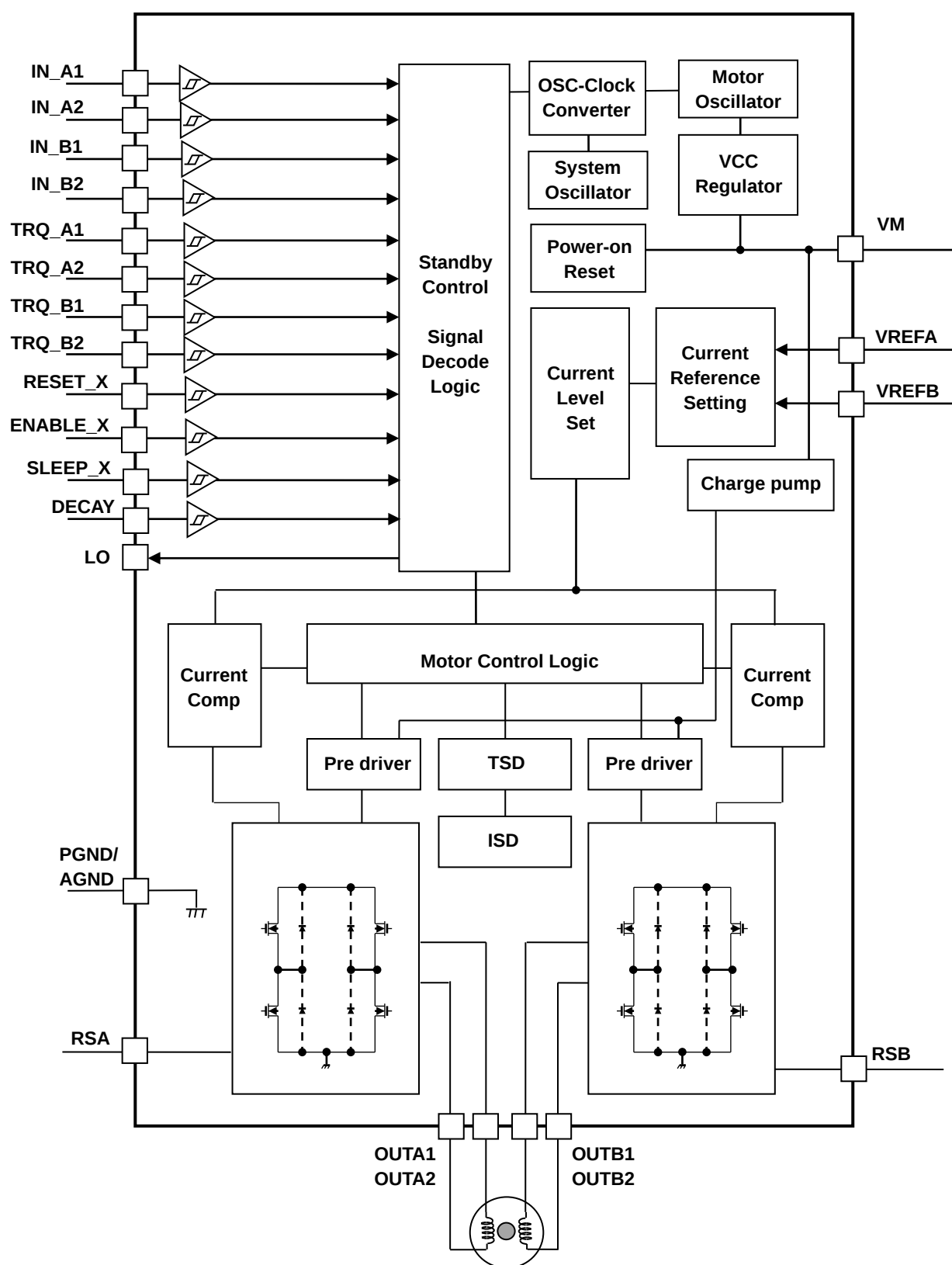
Figure 4 Block diagram
