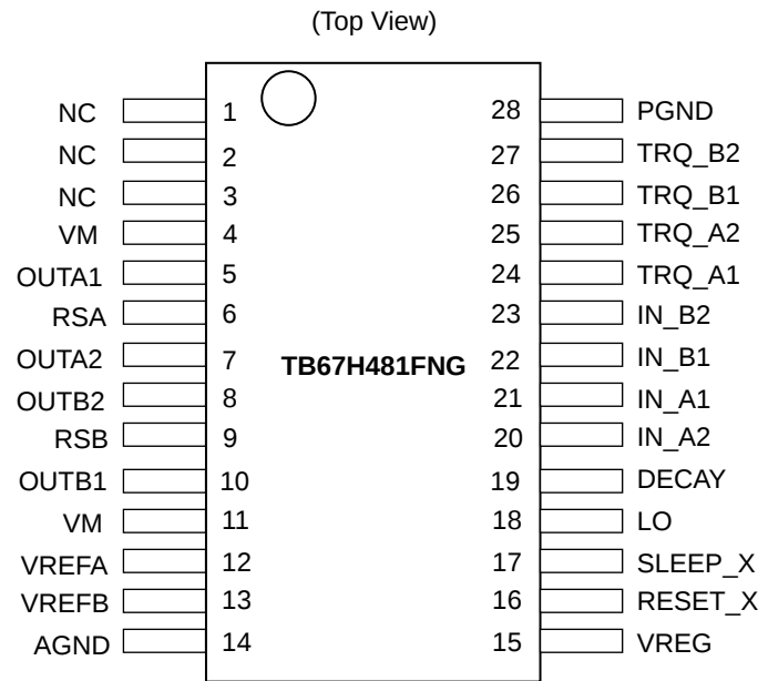
Figure 3 Pin Assignment
