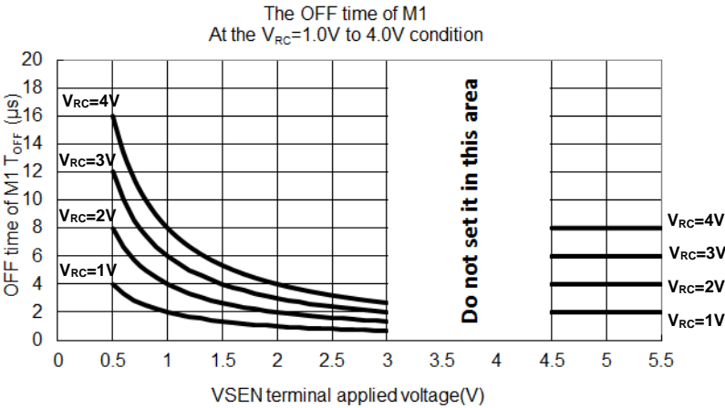
Figure 8 Off time Vs V RC V SEN
