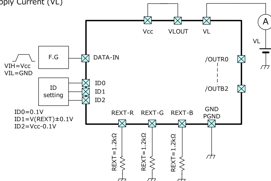
Test Circuit 3 Supply Current (VL)
