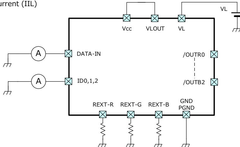
Test Circuit 2 Input Current (IIL)
