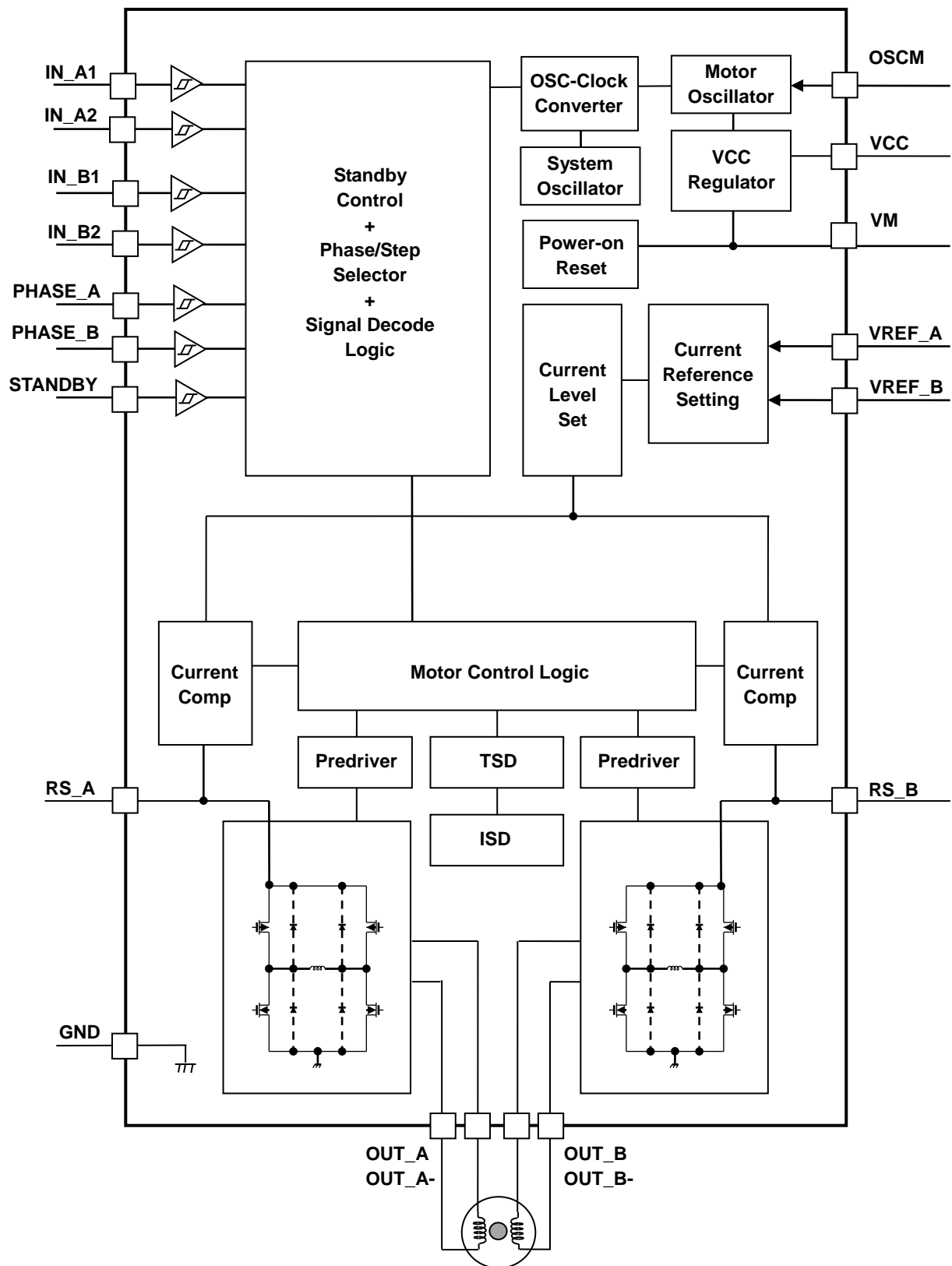
TB62261FTAG Block diagram
