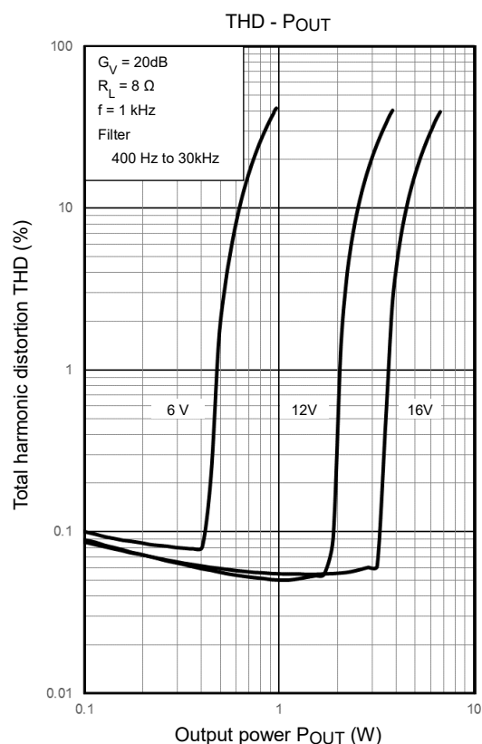
Figure 9 Total Harmonic Distortion by Power Supply Voltage
