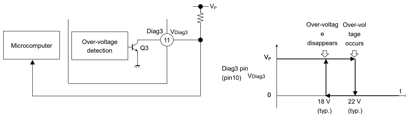
図 9 Over-Voltage Detection
