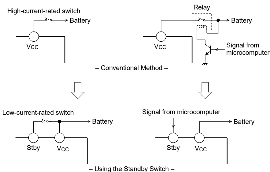
Figure 2 Standby Switch
