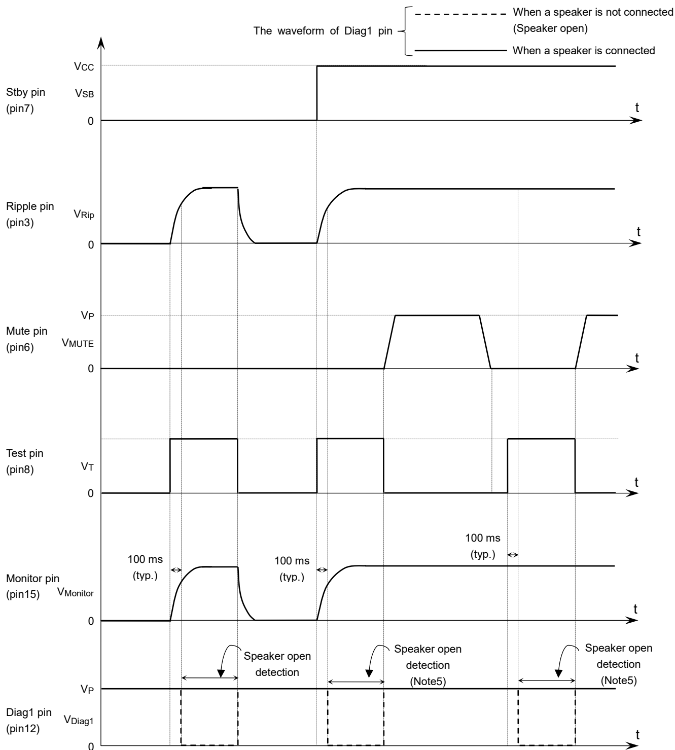
Figure6 Speaker Open Detection Sequence
