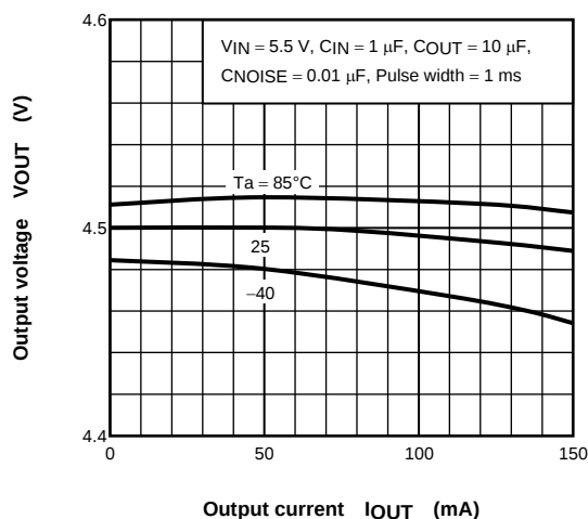
(TAR5SB45) I_{OUT} - V_{OUT}
