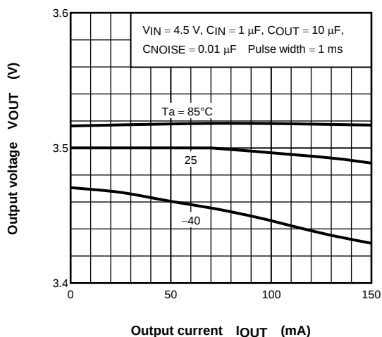
(TAR5SB35) I_{OUT} - V_{OUT}
