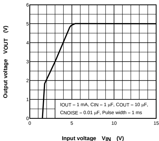
(TAR5SB50) V_{OUT} - V_{IN}
