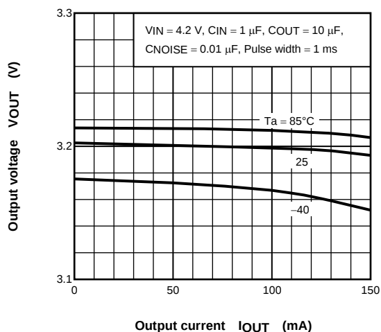
(TAR5SB32) I_{OUT} - V_{OUT}
