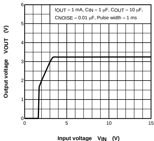
(TAR5SB32) V_{OUT} - V_{IN}
