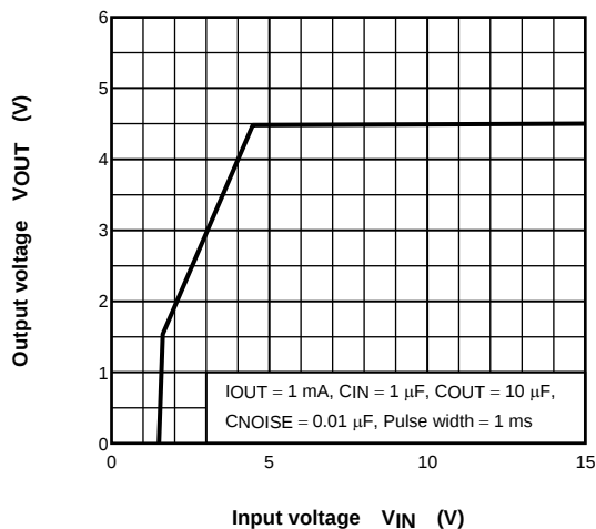
(TAR5SB45) V_{OUT} - V_{IN}
