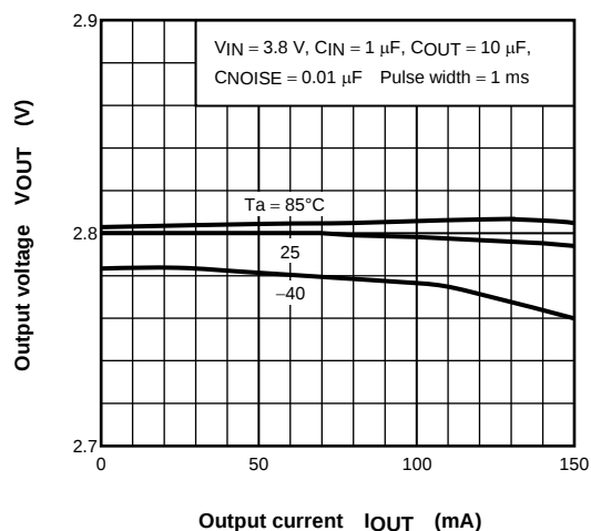
(TAR5SB28) I_{OUT} - V_{OUT}
