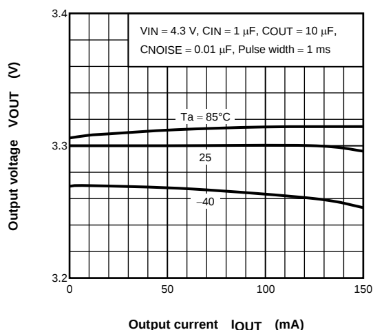
(TAR5SB33) I_{OUT} - V_{OUT}
