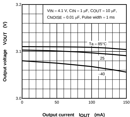
(TAR5SB31) I_{OUT} - V_{OUT}
