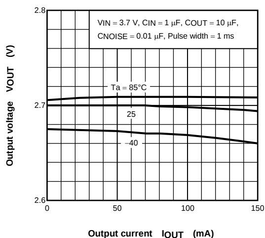
(TAR5SB27) I_{OUT} - V_{OUT}
