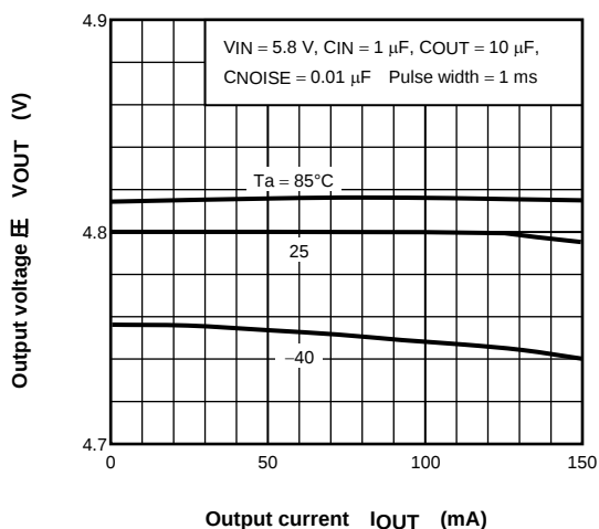
(TAR5SB48) I_{OUT} - V_{OUT}
