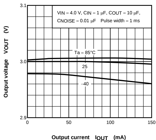
(TAR5SB30) I_{OUT} - V_{OUT}
