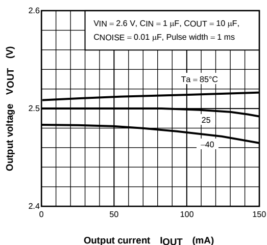
(TAR5SB25) I_{OUT} - V_{OUT}
