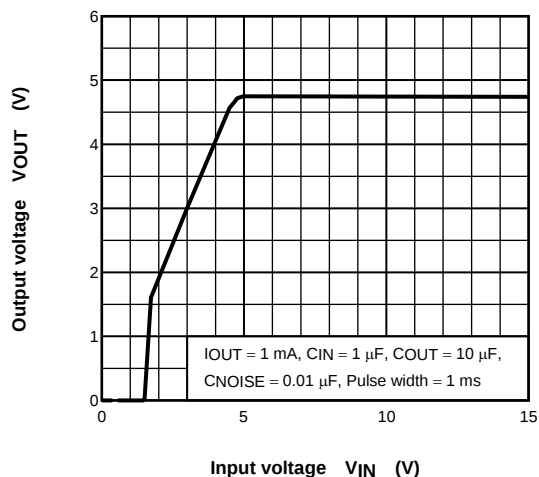
(TAR5SB48) V_{OUT} - V_{IN}
