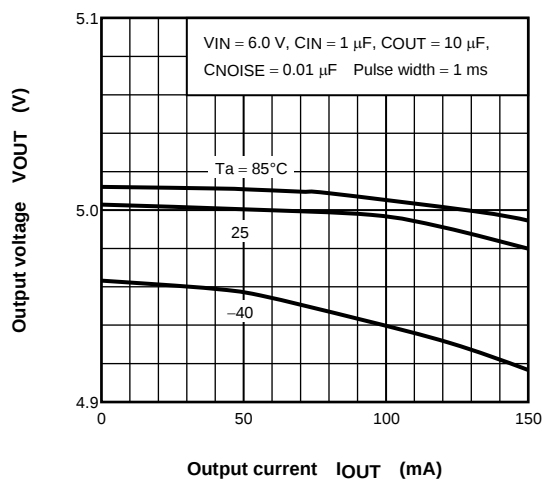
(TAR5SB50) I_{OUT} - V_{OUT}
