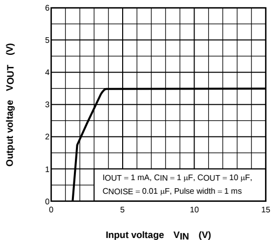
(TAR5SB35) V_{OUT} - V_{IN}
