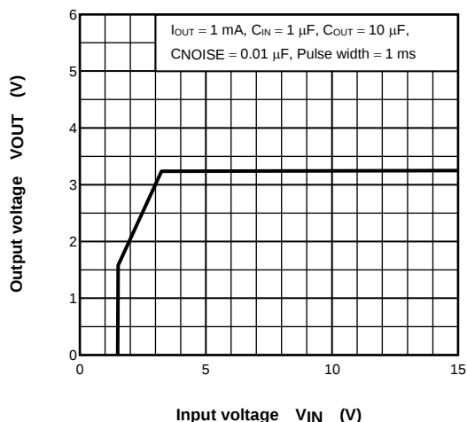
(TAR5SB33) V_{OUT} - V_{IN}
