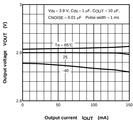
(TAR5SB29) I_{OUT} - V_{OUT}
