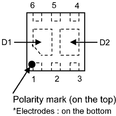
Fig. 6.2 Pin Condition(Top View)
