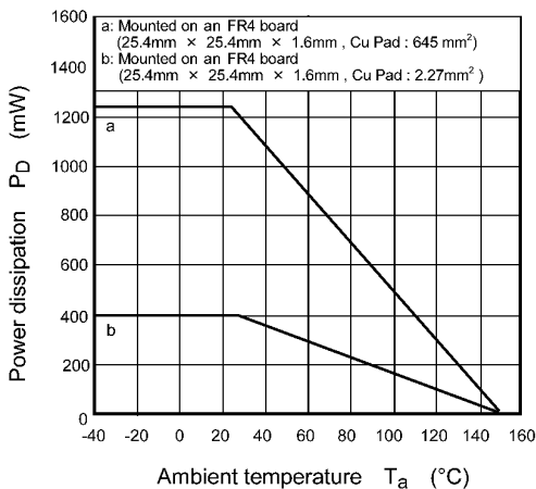
Fig. 8.11 P_D - T_a
